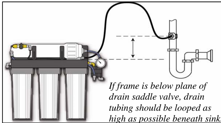
Figure 8, Drain Tubing Connection
