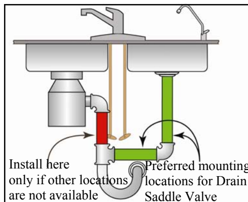
Figure 4, Drain Saddle mounting locations
