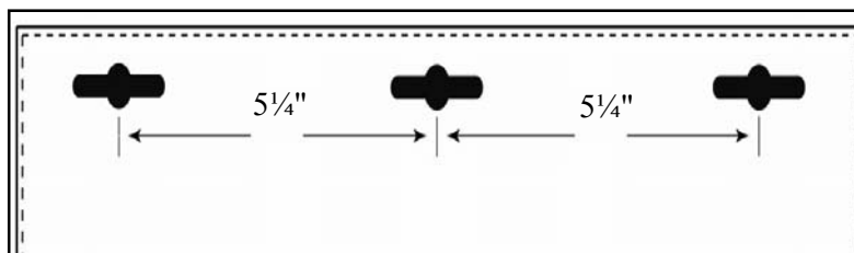
Figure 7, Spacing between keyholes (diagram not drawn to scale)
