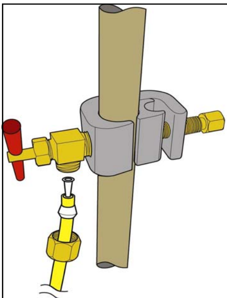
Figure 11, Connect tubing as diagrammed
