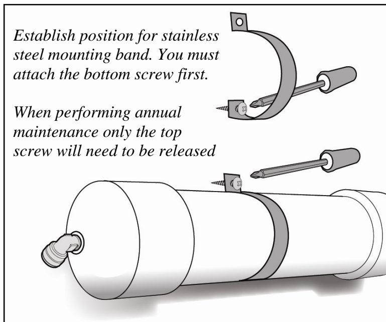
Figure 10, Mounting the Deionization Module
