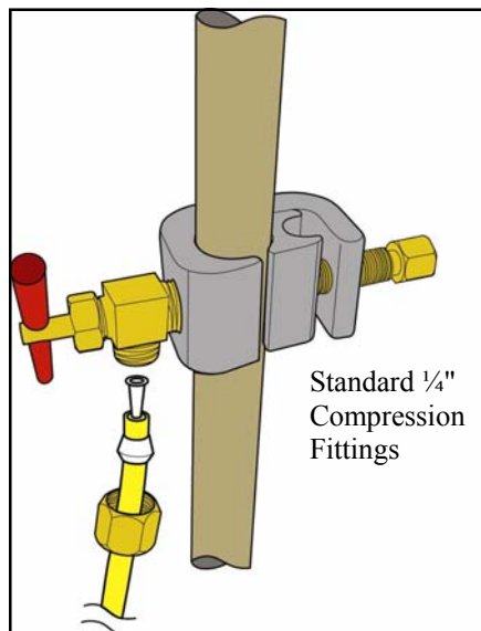
Figure 3, Feed Water Saddle Valve
