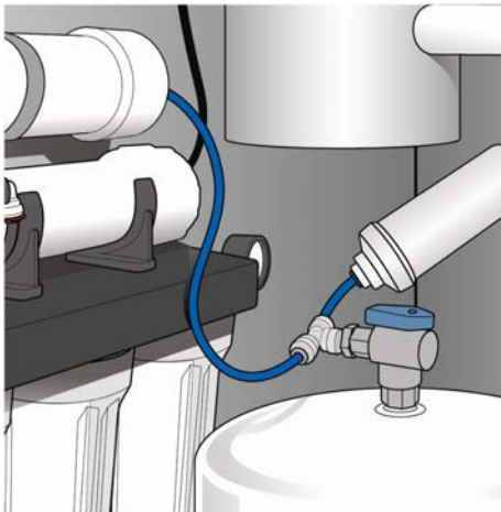
Figure 17, DI Module to Storage Tank Connection
