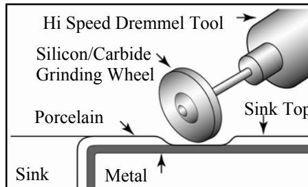
Figure 2, Using a Dremmel® Tool to Remove Porcelain
