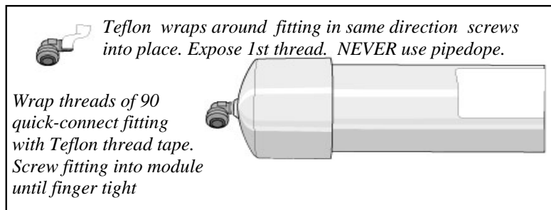
Figure 9, Installation of 90° Speedfit Fittings into Deionization Module
