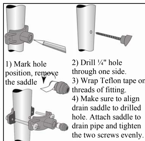
Figure 5, Mounting the Drain Saddle Valve
