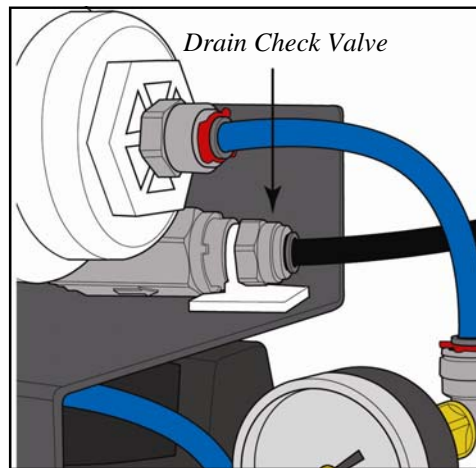
Figure 13, Drain Line Connection
